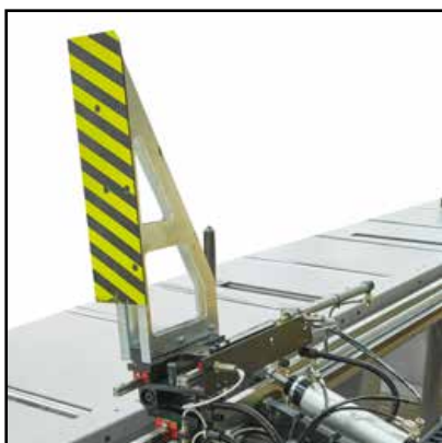
Motorized measurement length stop (Optional)
